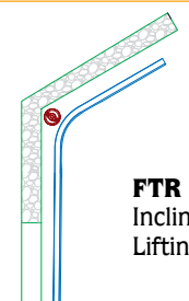
RES 100 Low headroom lift with spring assembly at rear
