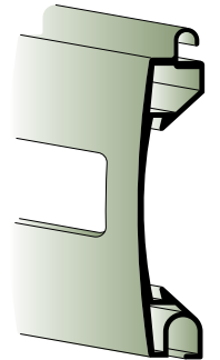
TEX - 77 Extruded Aluminum Slat with Window
