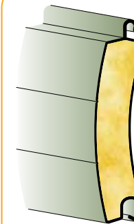
PCB (77 - 95) PU filled Painted Steel Slat
